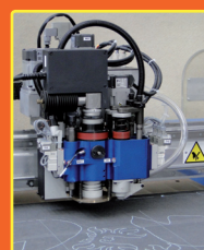
Testa multi utensile Multi-tool cutting head
